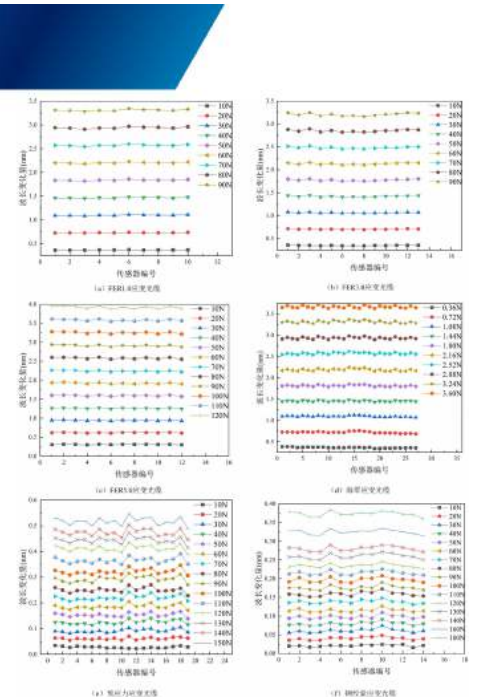
Figure 4. FRP strain-sensing cable design and calibration. Six cable structures were compared to evaluate strain transfer uniformity and robustness.
