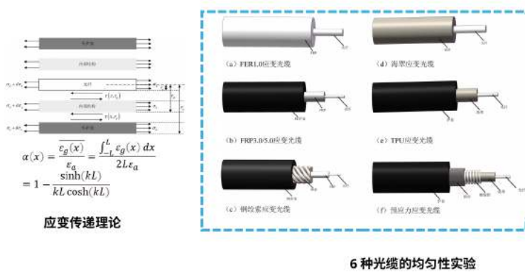
Figure 4. FRP strain-sensing cable design and calibration. Six cable structures were compared to evaluate strain transfer uniformity and robustness.
